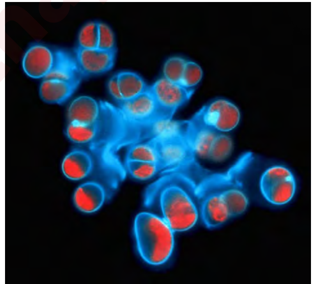
Figure 20.6 Chlorokybus extracellular matrix containing cellulose. These cells were treated with a compound that binds to cellulose and fluoresces bright white. (Photo: L. E. Graham)
