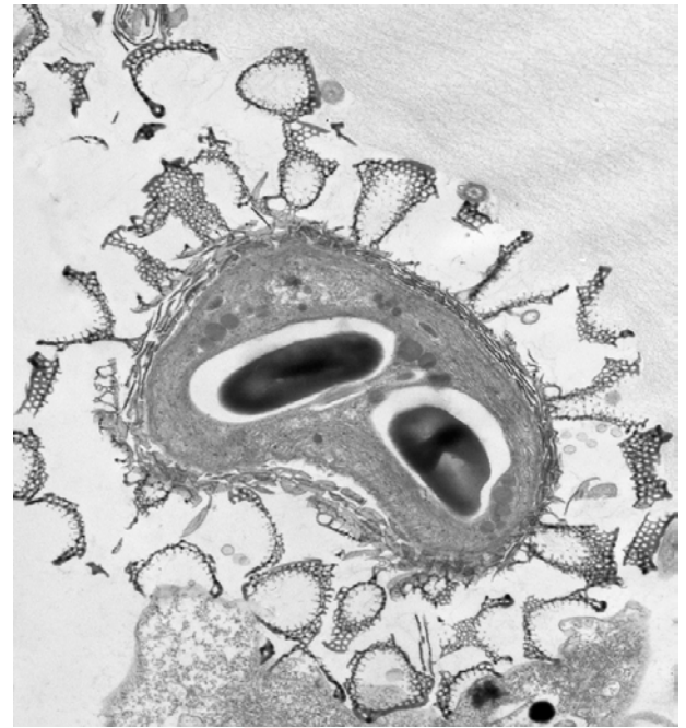
Figure 20.4 Mesostigma scale ultrastructure. TEM view of Mesostigma cell showing the multiple layers of scales as well as starch within the chloroplast. (Micrograph: E. Kim and L. E. Graham)
