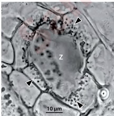
Figure 20.57 Coleochaete orbicularis transfer cells. Cells that surround zygotes (Z) have numerous, localized wall projections (arrowheads). Production of such ingrowths appears to be induced by the presence of zygotes and is additional evidence of chemical interaction between parent and progeny. Similar wall ingrowths occur at the interface of parent and progeny tissues in land plants, and the cells in which they occur are known as placental transfer cells. (From Graham and Wilcox 1983)
