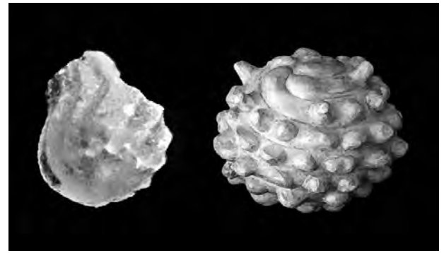
Figure 20.73 Fossil gyrogonites. On the left is an image of a fossil known as Ampullichara . On the right is a model made of a more complex gyrogonite fossil.
