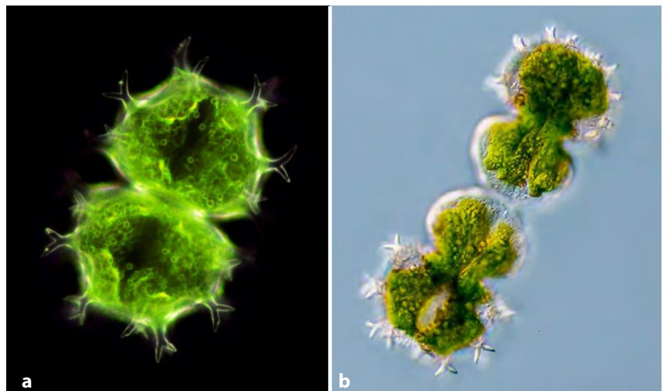
Figure 20.33 Xanthidium . This genus is characterized by three-dimensional protuberances on each of the semi-cells (a). In (b), a dividing cell is shown. Note that the characteristic protuberances have yet to form on the new semi-cells. (Photos: L. W. Wilcox)
